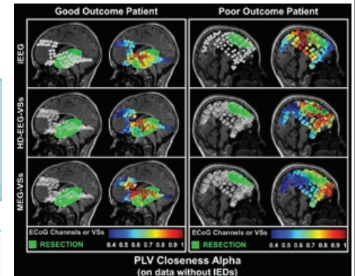
Fig. 4. FC analysis at patient's level. Heat map of PLV closeness estimated on data without IEDs in alpha frequency band for a 12-year-old male patient with good (left) and a 14-year-old male patient with poor (right) outcome.
