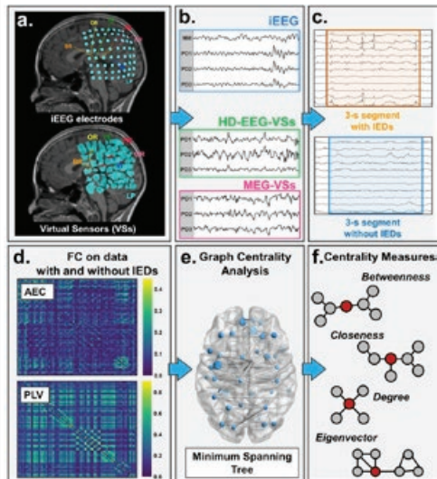
Fig. 1. Flow chart of methods. a) Virtual sensors (VSs) at iEEG locations; b) iEEG and VSs time-series filtered at (1-50) Hz; c) Selection of data with and without IEDs; d) AEC and PLV matrices, for each frequency band, type of activity (with and without IEDs) and signal (iEEG, HD-EEG-VSs, MEG-VSs); e) General representation of MST to generate sub-graphs; and f) MST's centrality measures.
